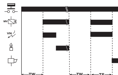
BOILERS WITH NATURAL DRAUGHT DBI version
