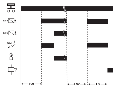
BOILERS WITH NATURAL DRAUGHT IP version
